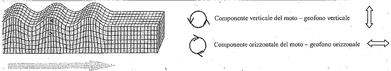
Rayleigh Wave
